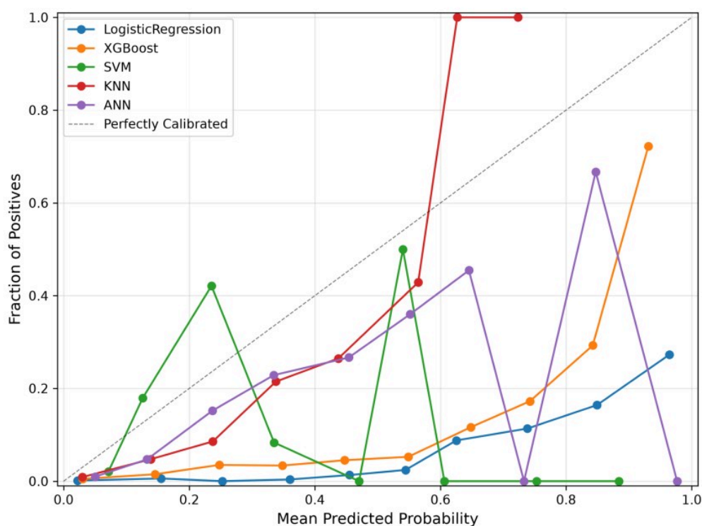
Figure 4. Probability calibration curves for all five models. The diagonal represents perfect calibration
