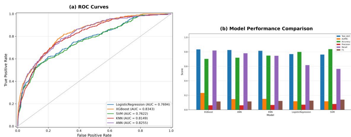
Figure 1. (a) ROC curves for all five models on the test set. (b) Performance comparison across six evaluation metrics
