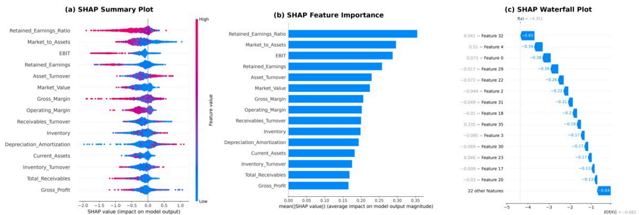
Figure 2. (a) SHAP beeswarm summary plot. (b) Global feature importance (mean |SHAP|). (c) Waterfall plot for a single prediction
