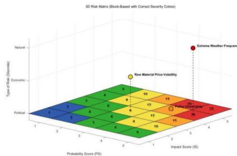
Figure 4. Three-dimensional probability-impact matrix
