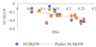
Figure 1. ESG line fit plot
