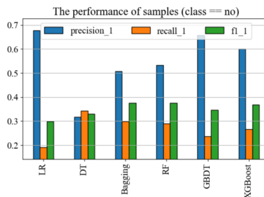
Figure 8: The performance of samples(class==no)
