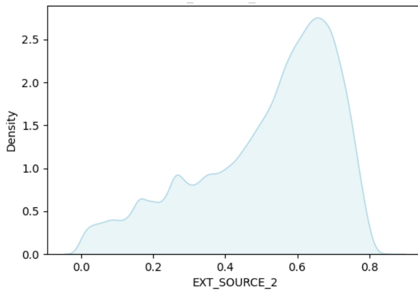
Figure 1: Credit score distribution map obtained using Random Forest model
