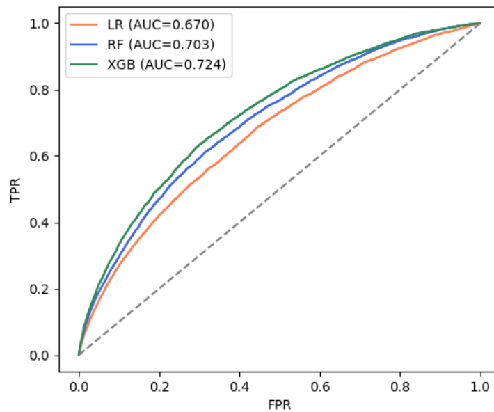
Figure 4: ROC curve obtained using XGboost model
