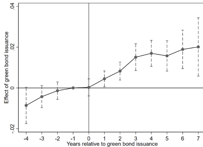
Figure 1: Parallel test
