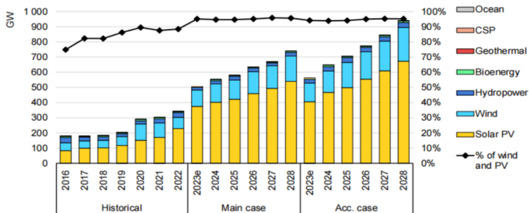
Figure 1: Renewable electricity capacity additions by technology and segment [1].
